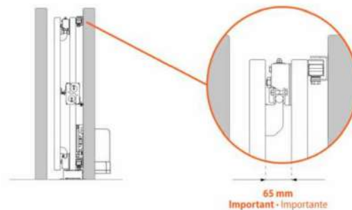
Kit autoportante telescopico apertura 3,5-8 m Telescopic cantilever kit opening 3,5-8 m
